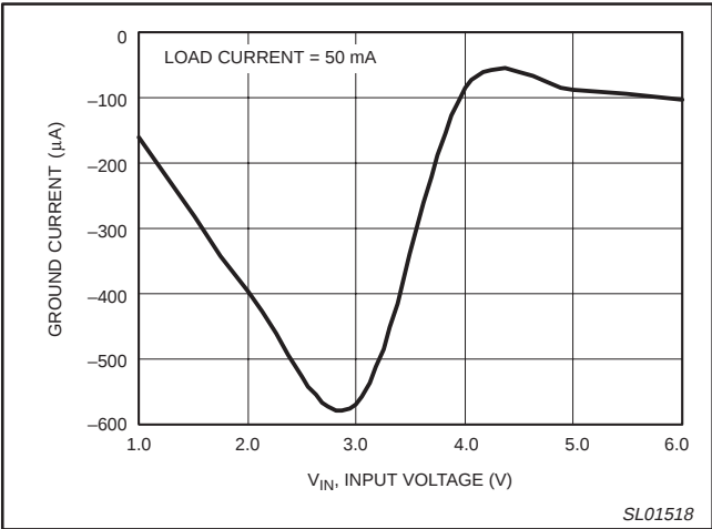
Figure 6. Ground current versus input voltage with load.
